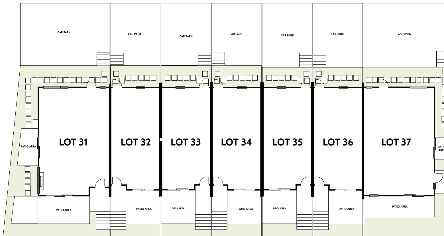
SITE PLAN
